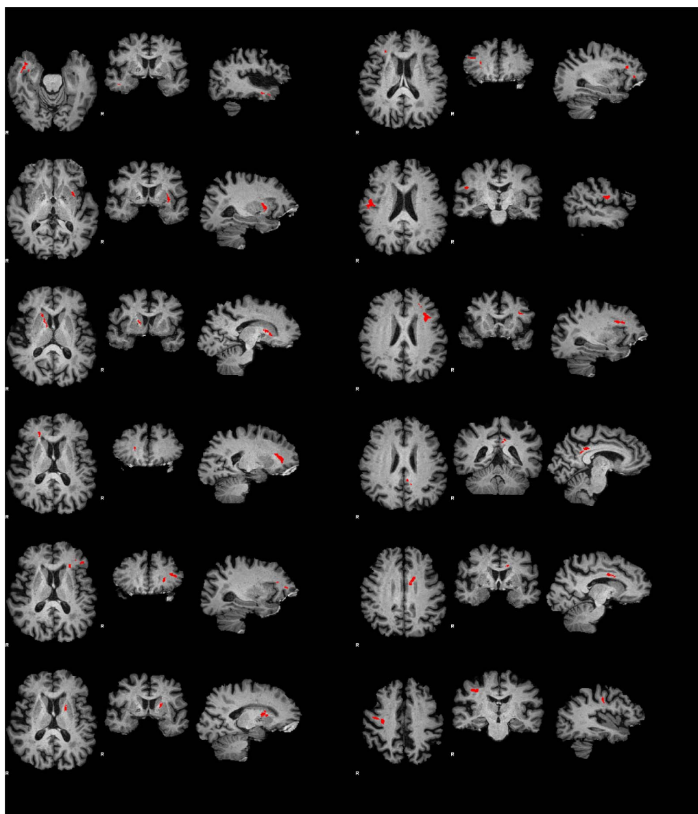
Fig. 3. Clusters of voxels (red) with significant correlations of FA and pulsatility index in left MCA. All correlations were negative: higher pulsatility is associated with lower FA. See Table 3 for summary of clusters in all examined arteries.
