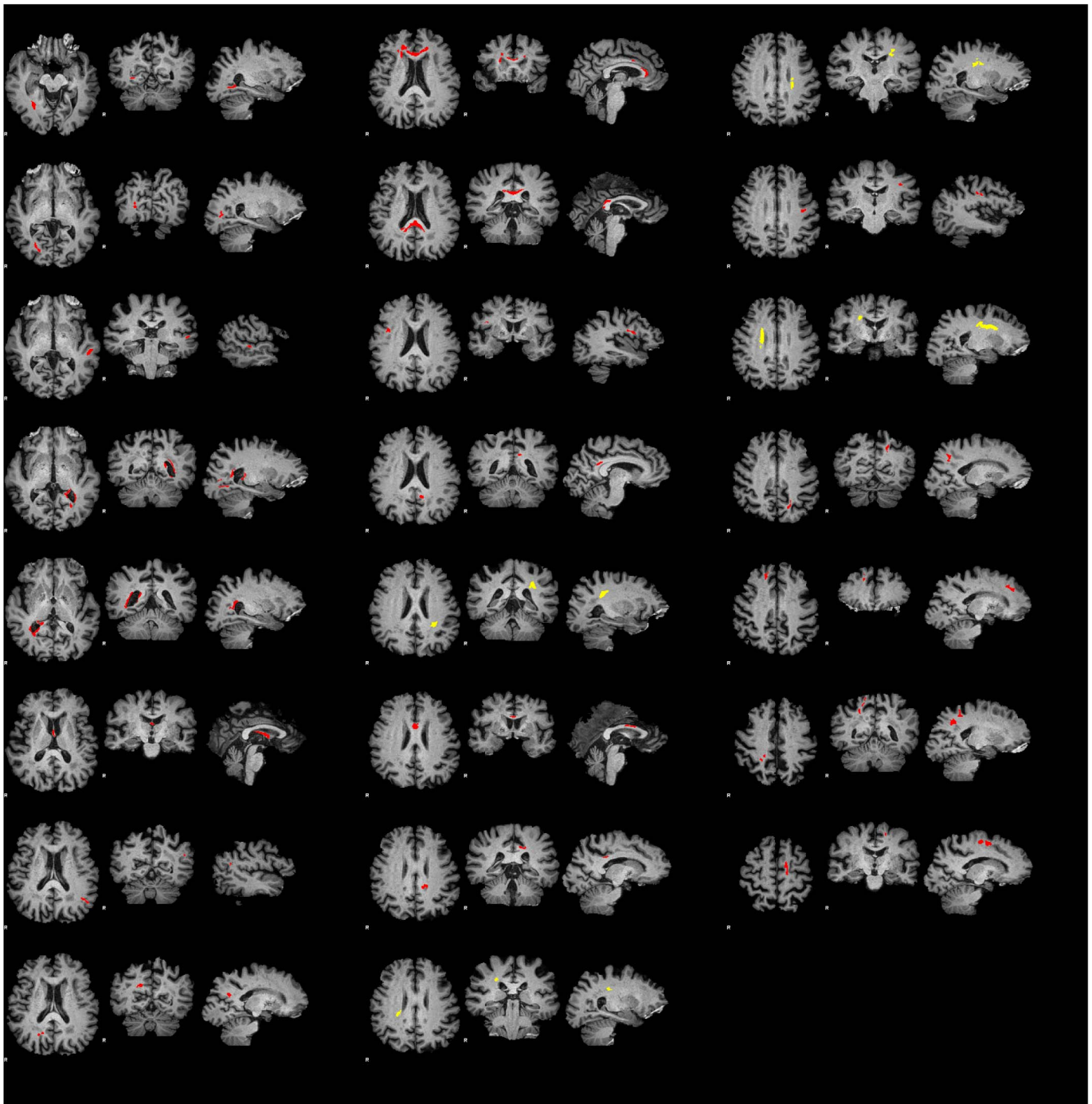
Fig. 2. Clusters of voxels with significant correlations of FA and age. Clusters with negative correlations where older age is associated with lower FA are marked in red. Those with positive correlations — in yellow.
