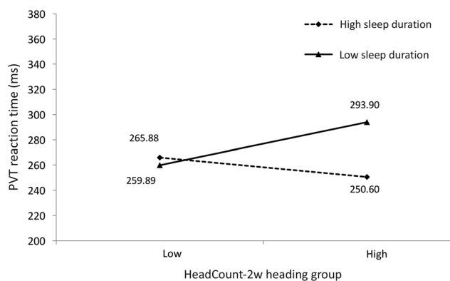
Fig. 1. Moderating effect of self-reported sleep duration on the relationship between recent head impact exposure (HeadCount-2w) and sustained attention (PVT, lower score = better performance).
